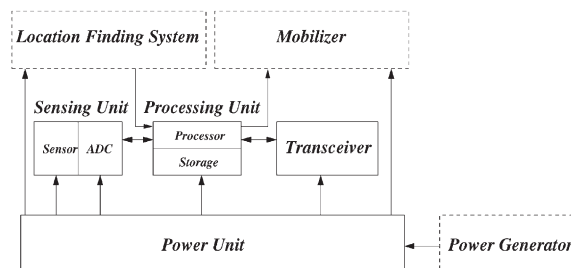
Fig. 1. The components of a sensor node.
